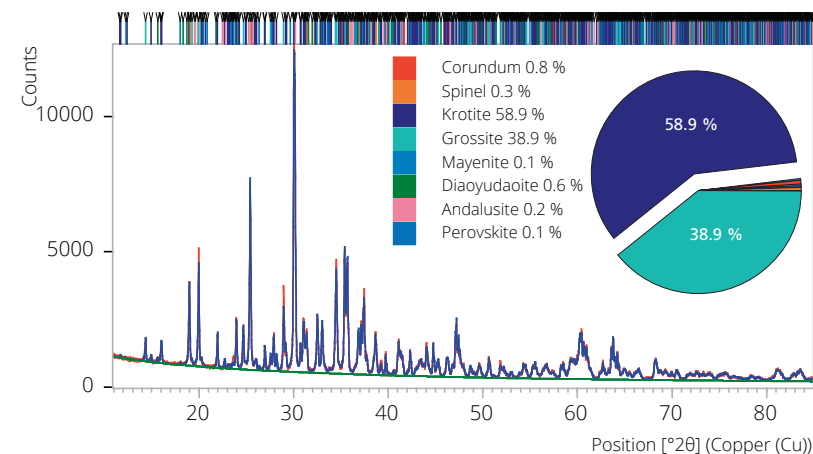
Rietveld refinement of high-temperature ceramic
